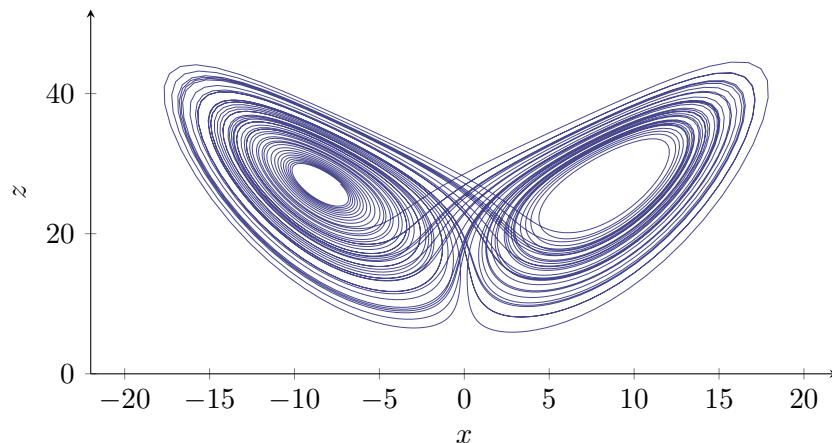
Figure 1.7.: A single trajectory of the Lorenz system (1.19), projected onto the xz -plane: the “butterfly” strange attractor. The curve never closes and never repeats, yet stays forever in a bounded region.
