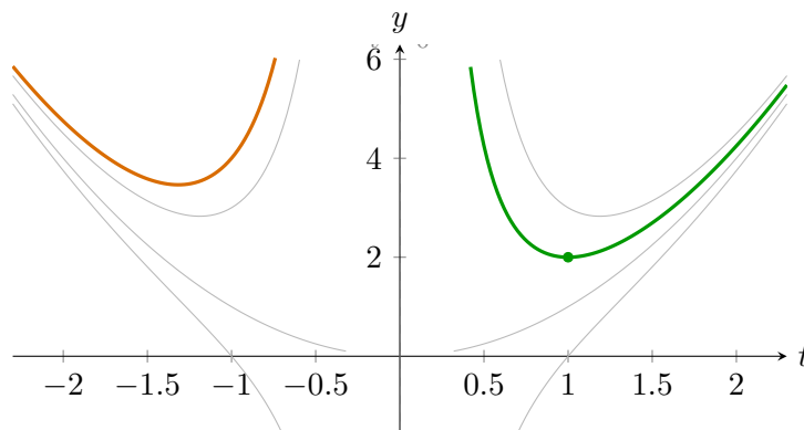
Figure 2.2.: No integral curve of ty' + 2y = 4t^2 crosses t = 0 (dashed): every curve with c \neq 0 blows up there. The green curve, c = 1 , is the solution of the IVP y(1) = 2 ; it lives only on t > 0 . The formula happens to be even in t , so the same shapes reappear for t < 0 (thin gray) — but the initial condition never touches that side, so the orange curve ( c = 3 ) would glue on just as legitimately as any other choice.
