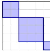
sizes (2, 3, 1) per = 2! 3! 1! = 12
