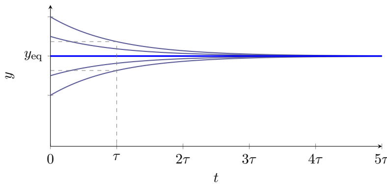
Figure 1.4.: Relaxation towards a stable equilibrium: every solution of (1.12) forgets its initial value exponentially, on the time scale \tau = 1/k .
