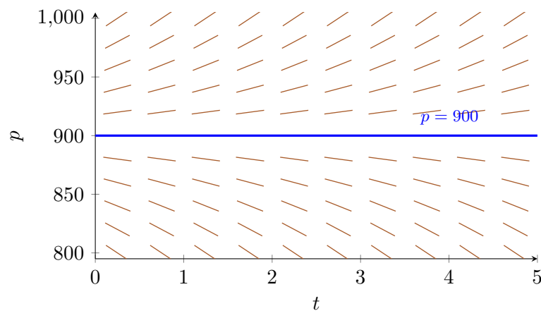
Figure 1.3.: Direction field and equilibrium solution of dp/dt = p/2 - 450 . Here the equilibrium p = 900 repels the other solutions.
