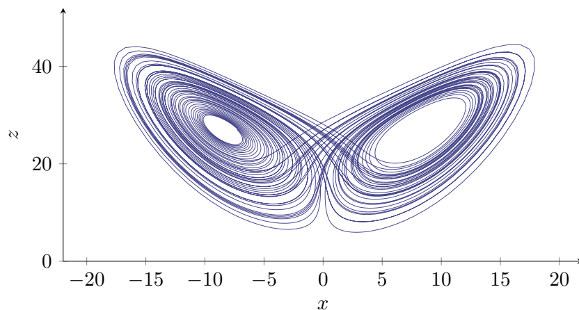
Figure 1.7.: A single trajectory of the Lorenz system (1.19), projected onto the xz -plane: the “butterfly” strange attractor. The curve never closes and never repeats, yet stays forever in a bounded region.
