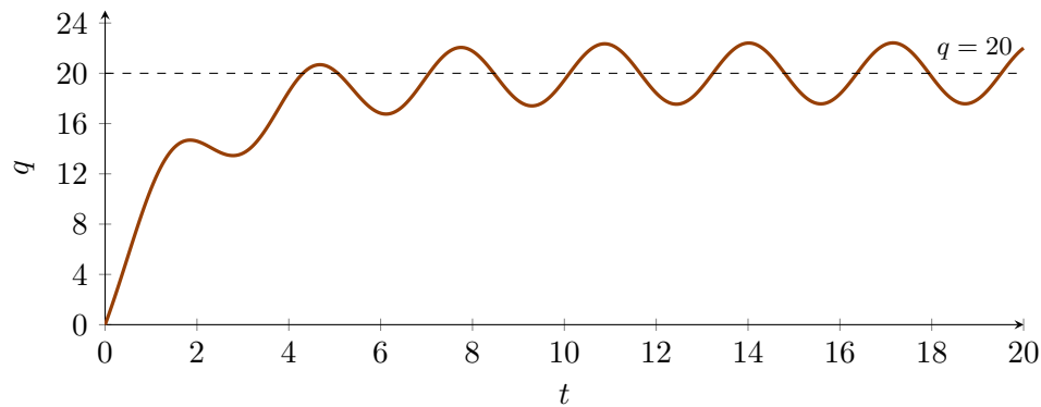
Figure 2.5.: Solution (2.20) of the pond problem q' + q/2 = 10 + 5 \sin(2t) , q(0) = 0 .
