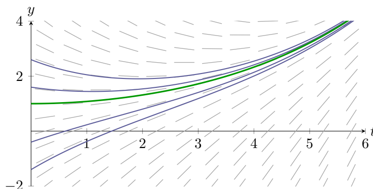
Figure 2.1.: Direction field and integral curves of y' + \frac{1}{2}y = \frac{1}{2}e^{t/3} ; the green curve is the solution through (0, 1) .
