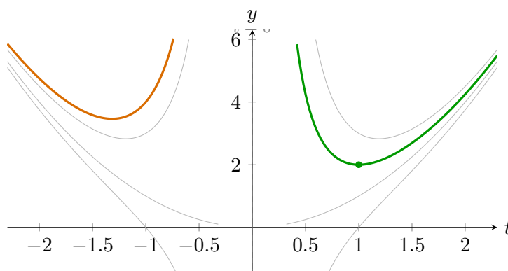
Figure 2.2.: No integral curve of ty' + 2y = 4t^2 crosses t = 0 (dashed): every curve with c \neq 0 blows up there. The green curve, c = 1 , is the solution of the IVP y(1) = 2 ; it lives only on t > 0 . The formula happens to be even in t , so the same shapes reappear for t < 0 (thin gray) — but the initial condition never touches that side, so the orange curve ( c = 3 ) would glue on just as legitimately as any other choice.
