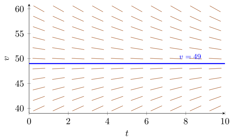
Figure 1.2.: Direction field and equilibrium solution of dv/dt = 9.8 - v/5 . The equilibrium v = 49 attracts the other solutions.
