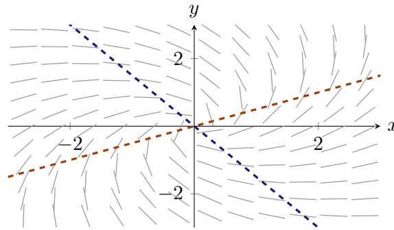
Figure 2.3.: Direction field of the homogeneous equation y' = (x+y)/(x-y) . Along each dashed ray y = vx the slope is the same constant g(v) — this is what “homogeneous” means.
