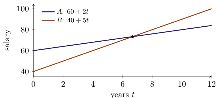
Figure 1.1.: The static comparison (values at t = 0 ) and the dynamic comparison (slopes) give opposite answers.
