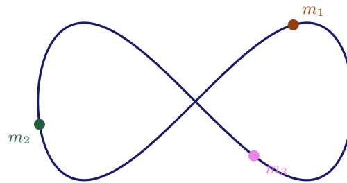
Figure 1.6.: The figure-eight orbit of the three-body problem (schematic, drawn as a lemniscate): three equal masses travel the same closed curve, spaced one third of a period apart. Discovered numerically by Moore (1993); existence proved by Chenciner and Montgomery (2000).
