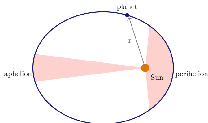
Figure 1.5.: The two-body problem: an elliptical orbit with the Sun at a focus. The two shaded regions have equal area and are swept out in equal times — so the planet moves fastest at perihelion.
