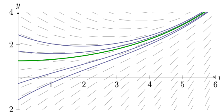
Figure 2.1.: Direction field and integral curves of y' + \frac{1}{2}y = \frac{1}{2}e^{t/3} ; the green curve is the solution through (0, 1) .
