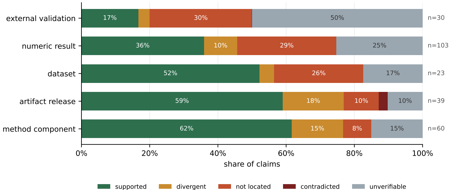
Do the artifacts support the claims? Discovery papers (n=32, 255 claims)
