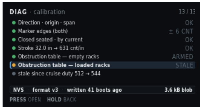
Figure 14. DIAG · calibration. Loaded table stale after cruise duty 512 → 544.
