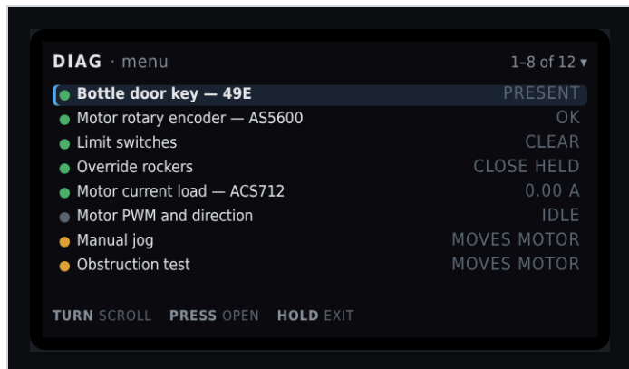
Figure 1. DIAG · menu. First window, bottle key selected.
