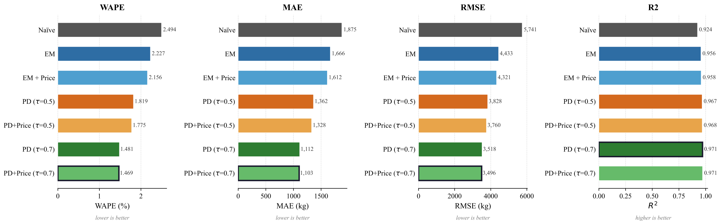
Figure 2. Model Performance Dashboard — Total Demand
