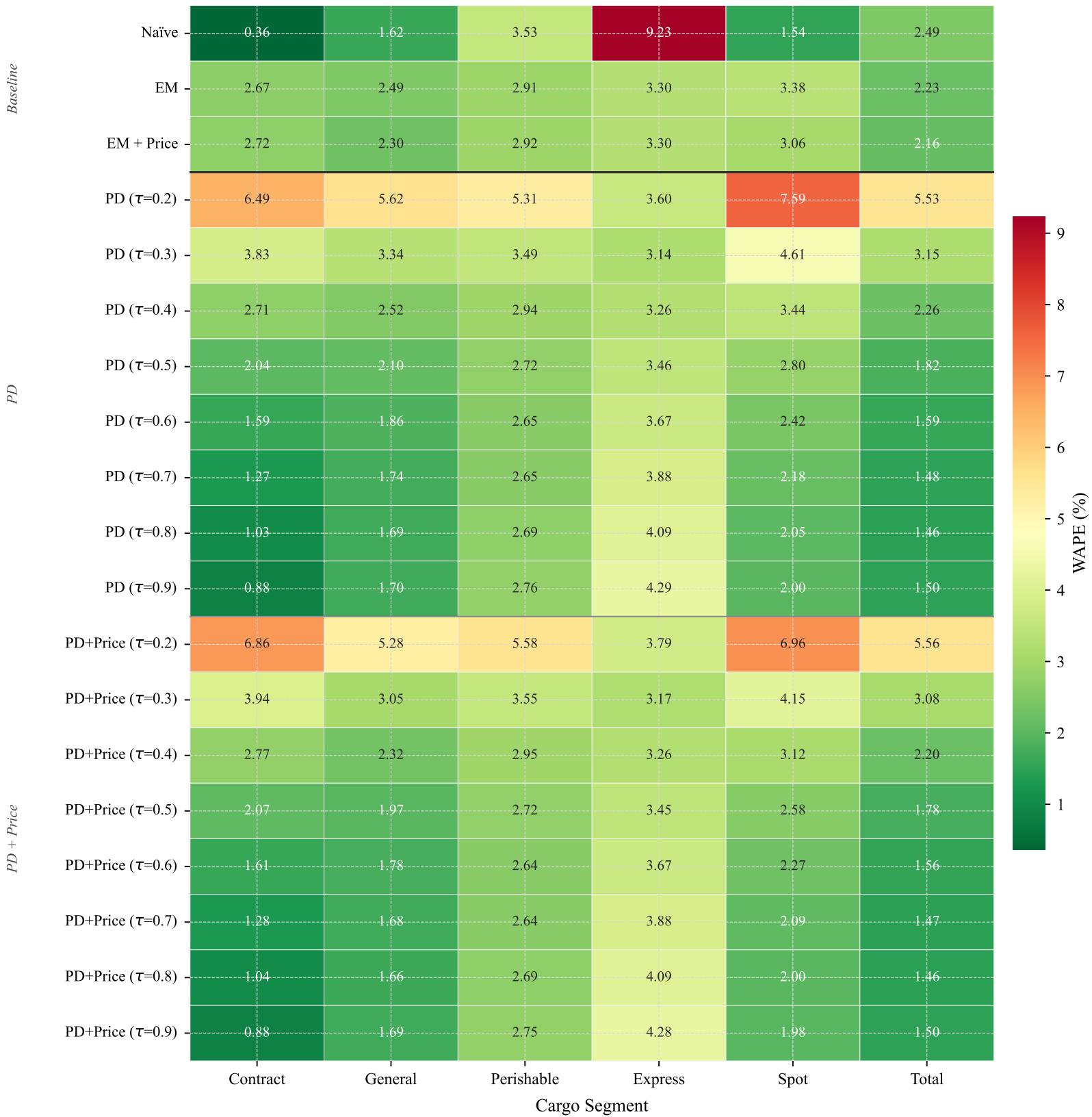
Figure 3. WAPE (%) Heatmap — All Models × Segments
