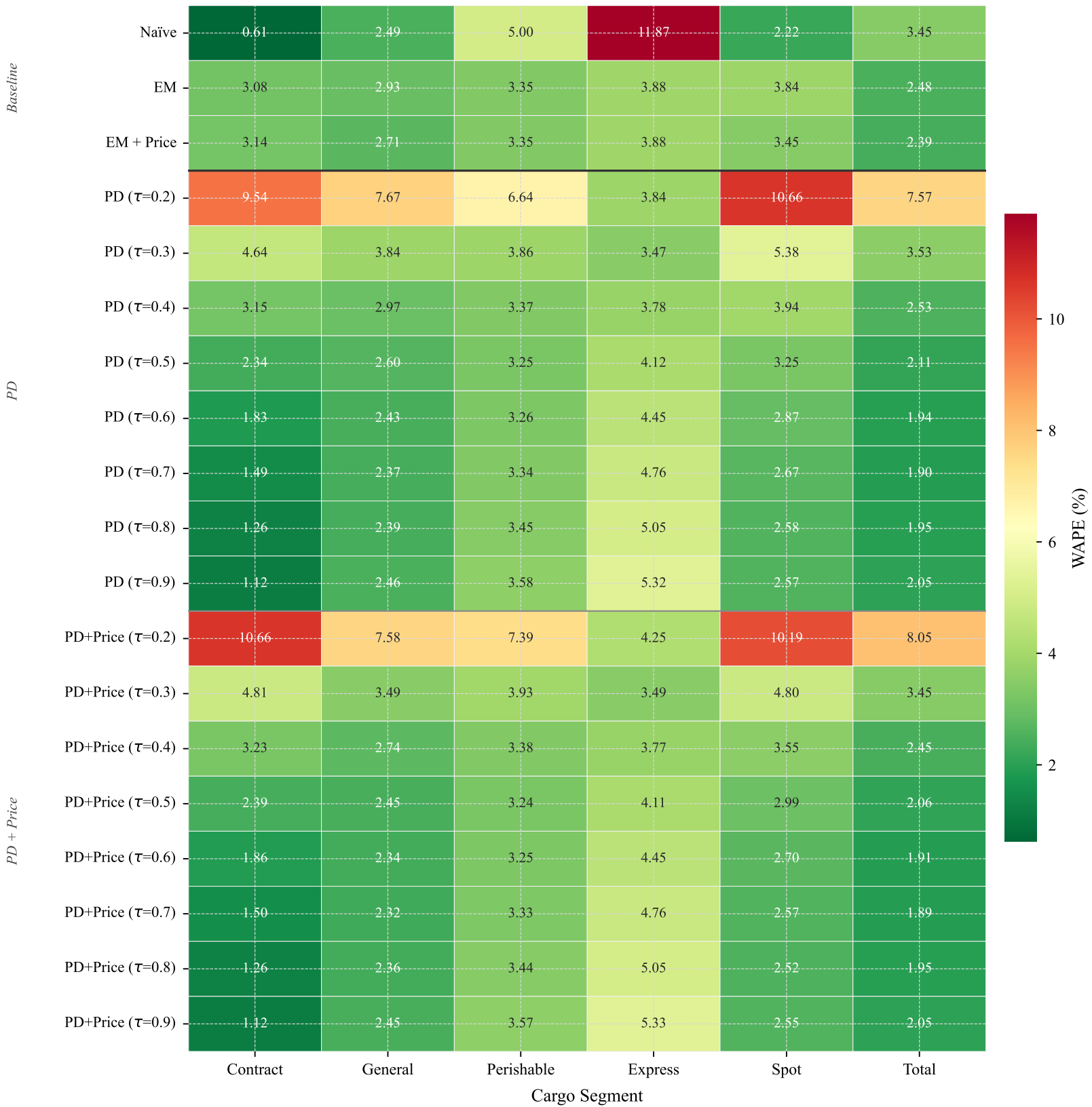
Figure 3. WAPE (%) Heatmap — All Models × Segments
