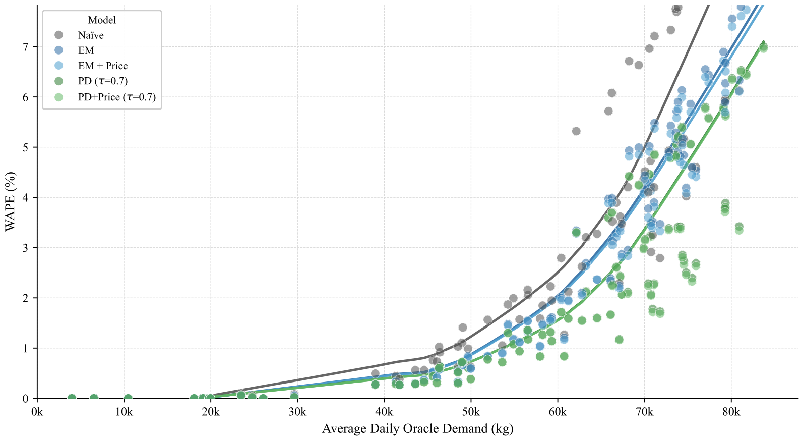
Figure 4. Model Effectiveness vs. Route Demand Volume
