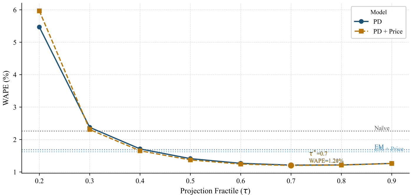
Figure 1. Sensitivity of WAPE to Projection Fractile \tau
