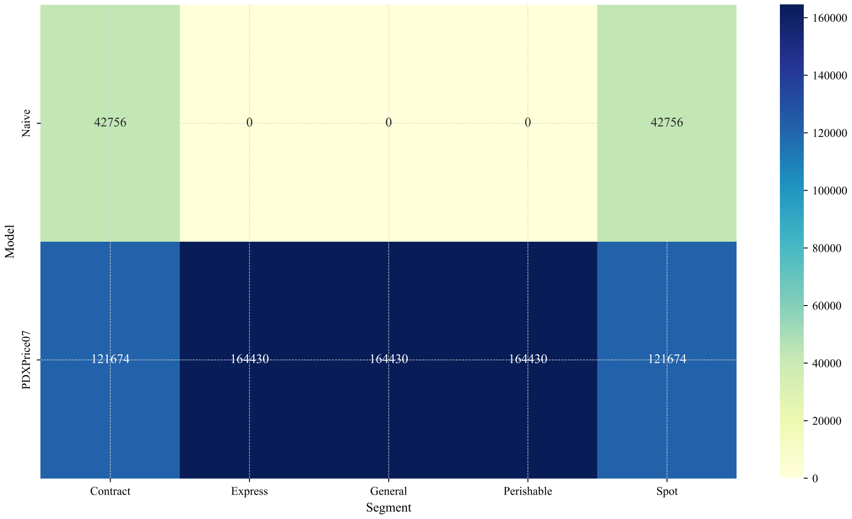
Figure 10. MoE Selection Distribution by Segment
