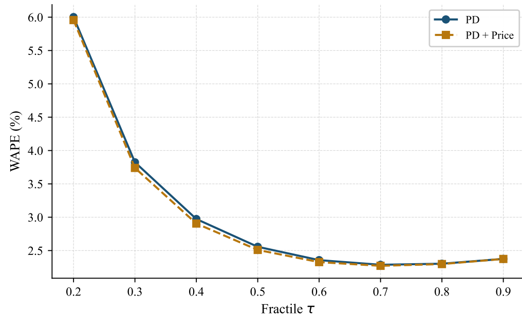
(a) Absolute WAPE by \tau
