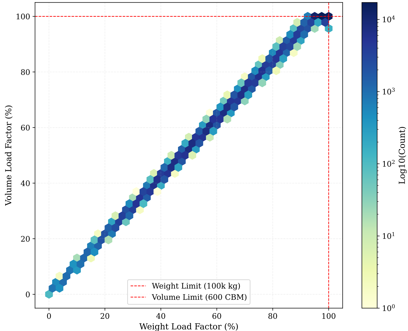
Physical Constraints: Joint Load Factor Distribution
