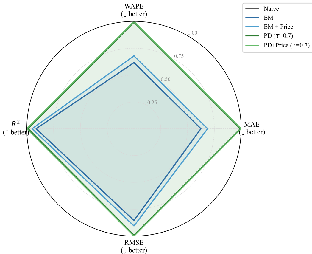
Figure 6. Normalised Performance Radar (outer edge = best)
