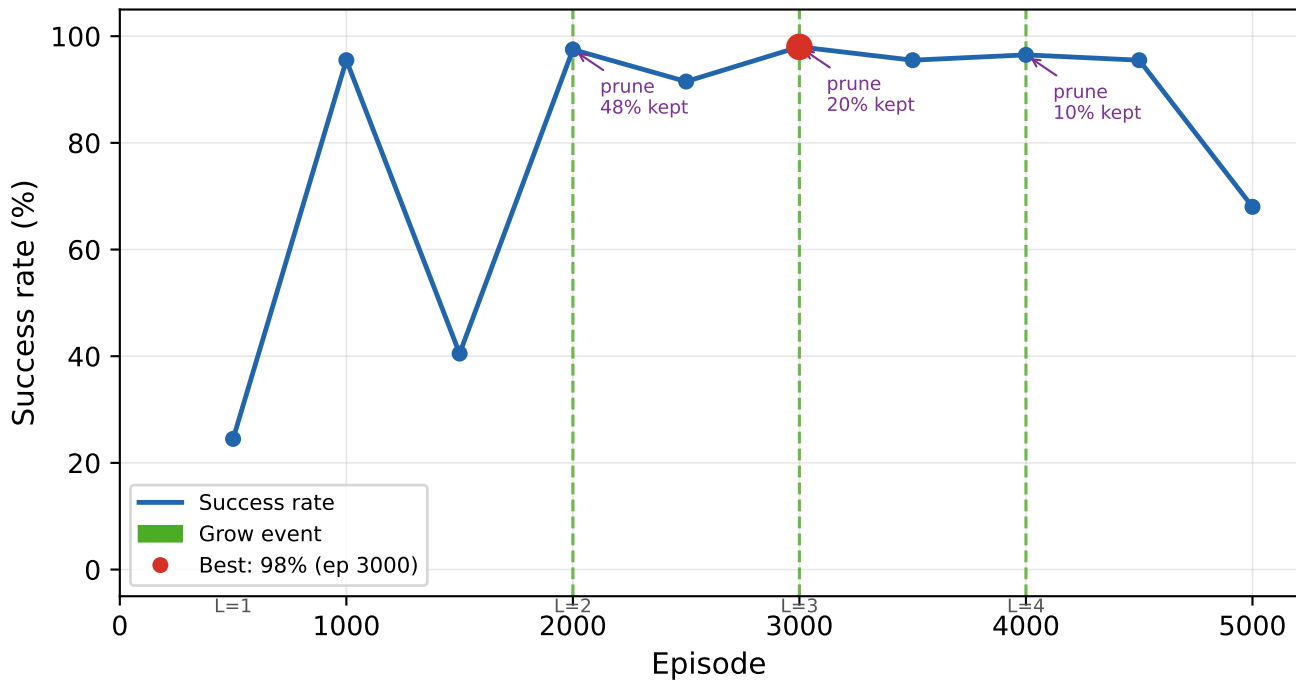
GPF Expected SARSA — Plume Navigation Training Curve
