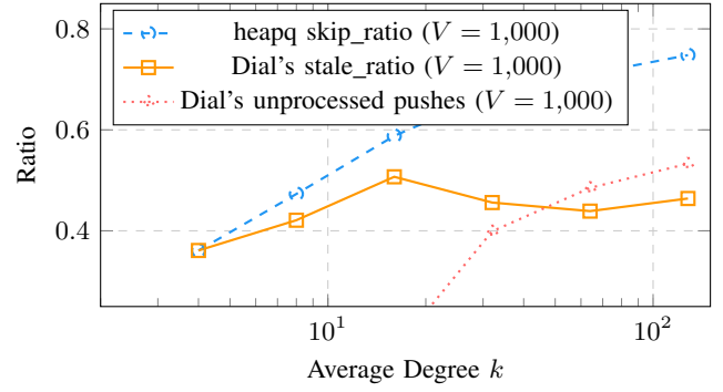
Fig. 6. heapq skip_ratio vs. Dial's stale_ratio and unprocessed-push fraction as functions of k (Experiment 8, V = 1,000 , log x -axis). As k grows, heapq's skip_ratio climbs monotonically while Dial's stale_ratio plateaus; the gap is absorbed by unprocessed pushes.
