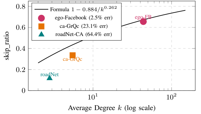
Fig. 7. \text{skip\_ratio} formula validated on SNAP datasets (Experiment 10). Black curve: formula (1) fitted on random graphs. Colored markers: measured \text{skip\_ratio} on real graphs.
