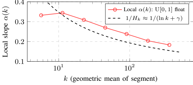
Fig. 3. Local slope \alpha(k) converges toward 1/H_k as k grows, consistent with the asymptotic \text{skip\_ratio} form 1 - c/H_k (theory_probe_v4, V = 3,000 , continuous float weights).
