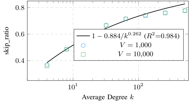
Fig. 1. skip_ratio vs. average degree k (log scale on x -axis). Circles: V = 1,000 ; squares: V = 10,000 . The fitted power-law curve (1) is plotted in black. Data pooled from Experiments 2 and A ( k \in [4, 512] ).
