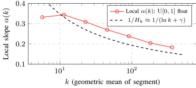
Fig. 3. Local slope \alpha(k) converges toward 1/H_k as k grows, consistent with the asymptotic skip_ratio form 1 - c/H_k (Exp. D4, V = 10,000 , continuous float weights).
