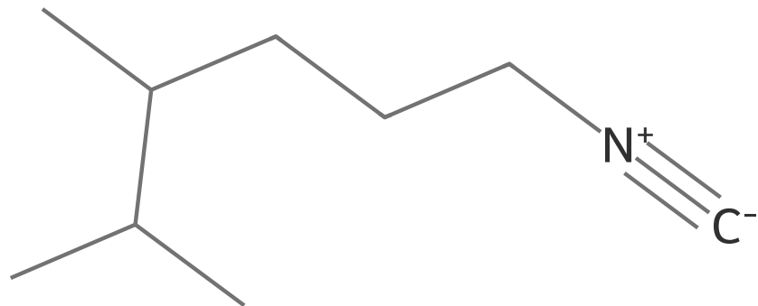
Isocyanide
