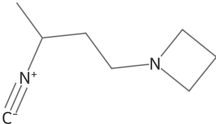
Isocyanide
