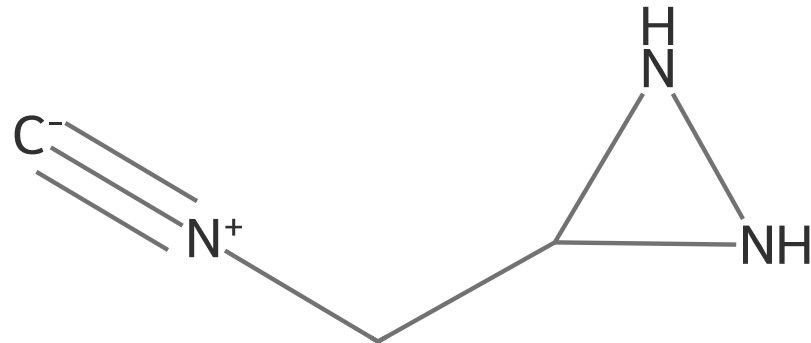
Isocyanide
