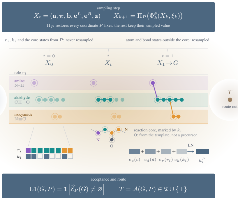
Figure 1: FORGE generates complete ionizable-lipid graphs within reaction-program coordinates. The reaction program specifies how molecular regions participate in an assembly without choosing their structures from a finite inventory. FORGE generates the complete molecular graph, verifies that the specified reaction reconstructs it, and recursively expands unavailable precursors until every branch terminates in evidence-qualified starting materials or the framework abstains. Exact replay and route closure are computational checks and do not establish experimental synthesis success.
