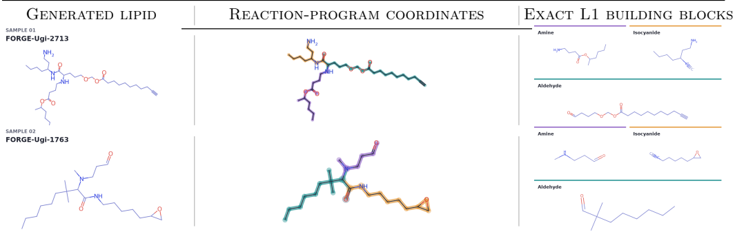
Figure 2: Deterministic examples of component-novel FORGE ionizable-lipid graphs. Each row is one seed-0 Ugi product with a unique exact-L1 decomposition and a recovered precursor constitution outside the method-visible training inventory. Left, the graph sampled jointly by FORGE; centre, precursor origins recovered by exact atom-mapped forward replay, halos marking the Ugi core; right, the exact precursor constitutions returned by the verifier. Purple denotes the amine-derived head, teal the aldehyde-derived body and tail, orange the isocyanide-derived tail and grey the assembly-introduced oxygen; these are semantic coordinates recovered by replay, not a vocabulary the model selects from. These are display examples, not experimental candidates, and exact-L1 replay is a structural diagnostic, not evidence of activity or synthesis success. Selection rule and the complete twelve-example atlas: Appendix F.
