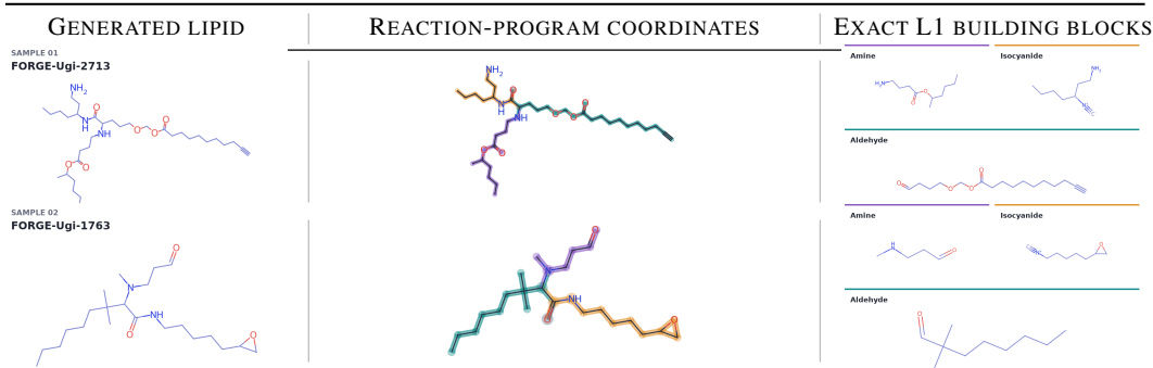
Figure 2: Exact Ugi products with recovered precursors absent from training. Each row contains a deterministic seed-0 product with a unique verified exact-L1 decomposition and a verifier-recovered precursor absent from training. Columns show the generated graph, atom-mapped origins and recovered precursors; halos mark the Ugi core and colours encode atom origin. These are structural examples, not evidence of activity or experimental synthesis success.
