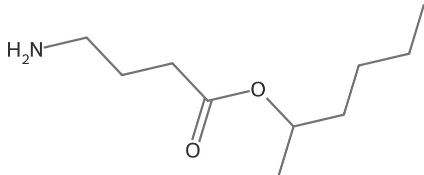
Amine
