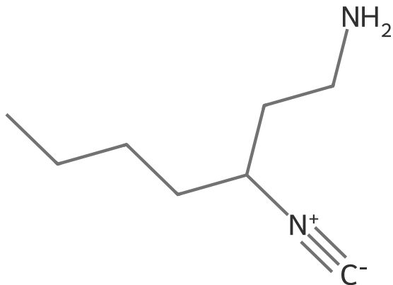
Isocyanide
