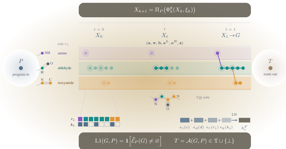
Figure 1: FORGE generates complete ionizable-lipid graphs within reaction-program coordinates. The reaction program specifies how molecular regions participate in an assembly without choosing their structures from a finite inventory. FORGE generates the complete molecular graph, verifies that the specified reaction reconstructs it, and recursively expands unavailable precursors until every branch terminates in evidence-qualified starting materials or the framework abstains. \Pi_P restores every coordinate the reaction program fixes and leaves the rest at the values just sampled. Haloed positions are the reaction-core positions k_i marks. In the Ugi-core inset, each atom carries the colour of the component it comes from; the carbonyl oxygen is grey because the assembly template introduces it and no precursor contributes it. Exact replay and route closure are computational checks and do not establish experimental synthesis success.
