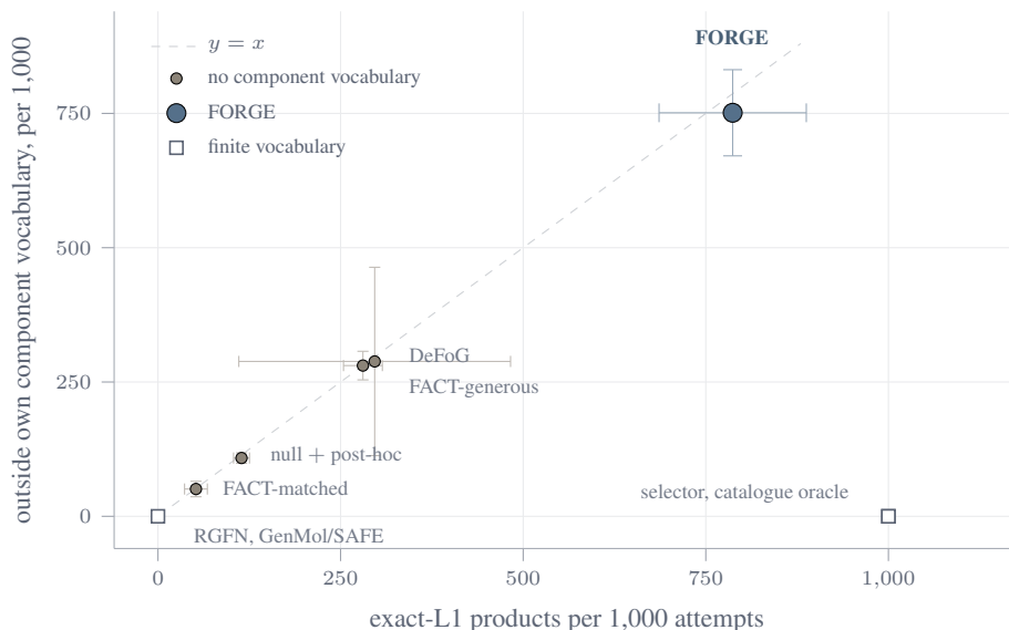
Figure 3: Reaction consistency and escape from a finite component vocabulary are separate axes. Common Ugi benchmark, per 1,000 generation attempts, mean and sample standard deviation over three seeds. Filled points are methods with no component vocabulary; they track y \approx x because almost every exact-L1 product they return is outside a vocabulary they do not have, so the diagonal is a property of that family rather than a result. Open markers are finite-vocabulary methods, whose outside-vocabulary yield is zero by Theorem B.3 rather than by measurement: every catalogue attempt uses catalogue components. The two families measure y against different references, so a filled point’s y is not comparable with an open point’s y ; the comparable component-novel metric against one fixed training catalogue is Table 8. What the figure shows is position along the diagonal: FORGE reaches 786.8 \pm 100.8 exact-L1 products, against 296.7 \pm 186.0 for the next open-ended method, while the two methods that exceed it on the horizontal axis cannot leave the floor.
