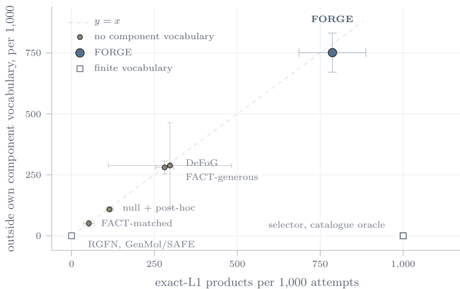
Figure 2: Reaction consistency and escape from a finite component vocabulary are separate axes. Common Ugi benchmark, per 1,000 generation attempts, mean and sample standard deviation over three seeds. Filled points are methods with no component vocabulary; they track y \approx x because almost every exact-L1 product they return is outside a vocabulary they do not have, so the diagonal is a property of that family rather than a result. Open markers are finite-vocabulary methods, whose outside-vocabulary yield is zero by Theorem E.3 rather than by measurement: every catalogue attempt uses catalogue components. The two families measure y against different references, so a filled point’s y is not comparable with an open point’s y ; the comparable component-novel metric against one fixed training catalogue is Table 9. What the figure shows is position along the diagonal: FORGE reaches 786.8 \pm 100.8 exact-L1 products, against 296.7 \pm 186.0 for the next open-ended method, while the two methods that exceed it on the horizontal axis cannot leave the floor.
