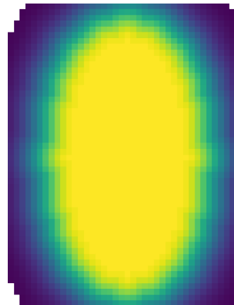
Score
