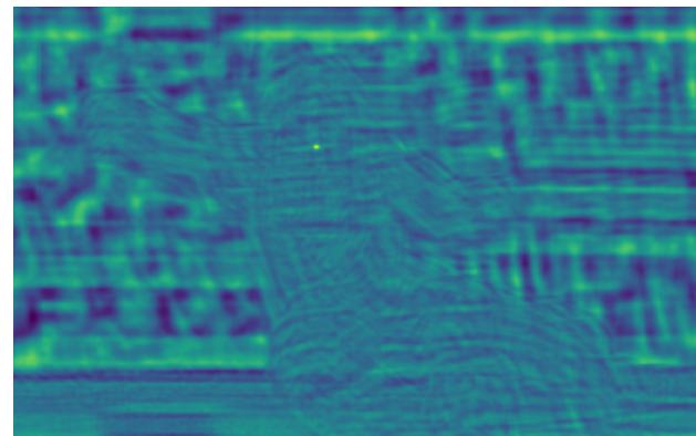
Score (Band-pass)
