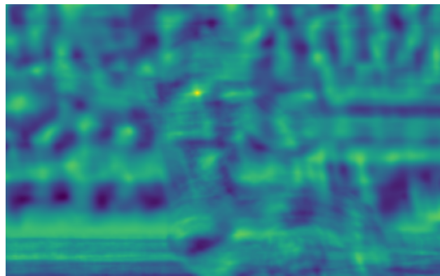
Score (Low-pass)
