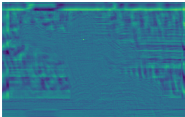
Score (High-pass)
