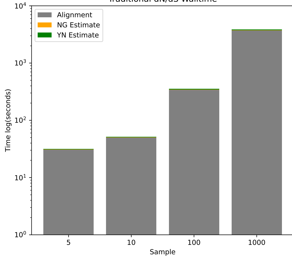
Traditional dN/dS Walltime
