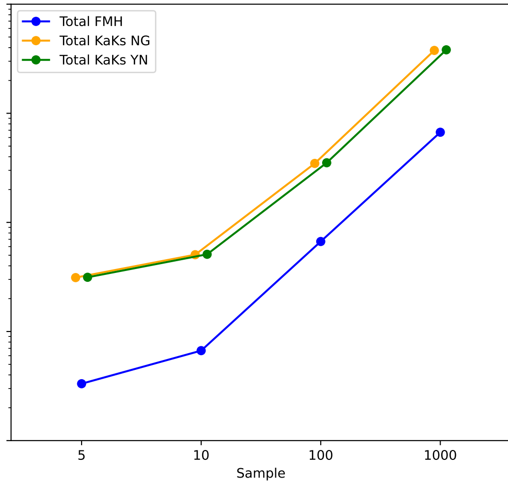
Traditional vs FMH dN/dS Walltimes
