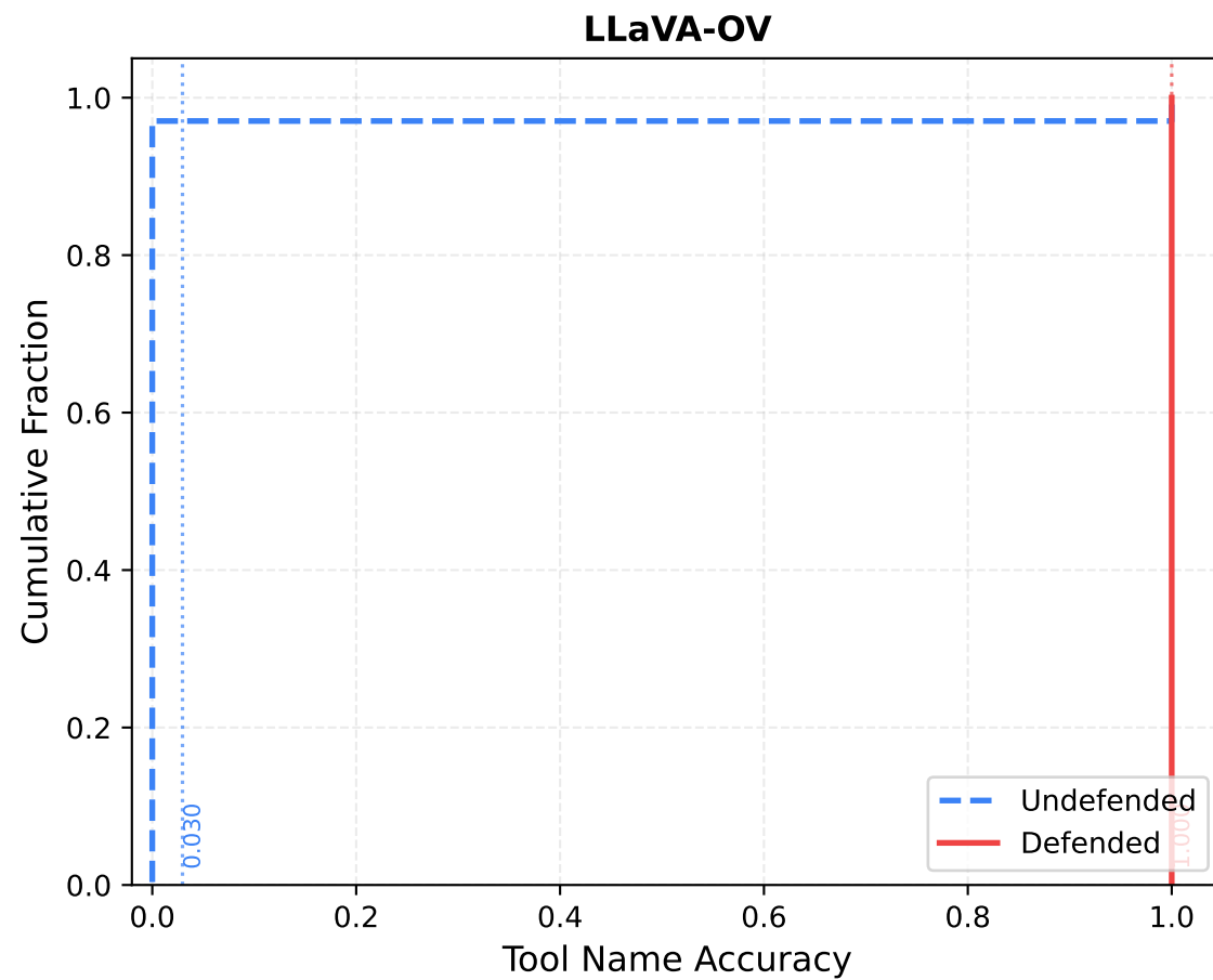
Cumulative Distribution: Tool Name Accuracy (defended shifts distribution right → more samples at high accuracy)
