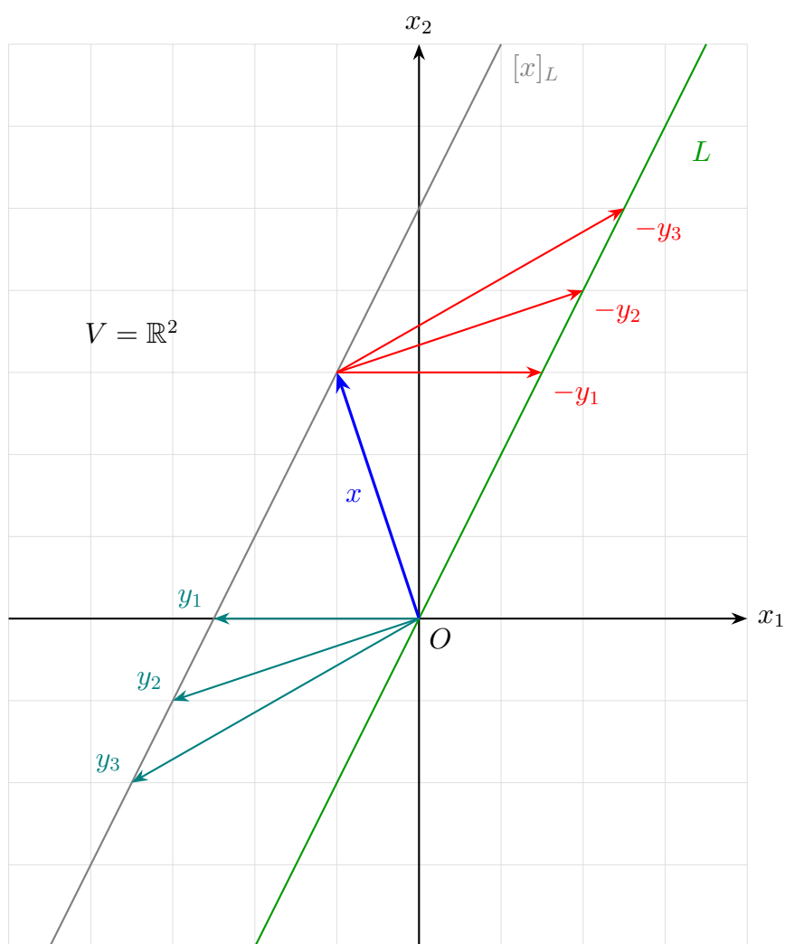
Slika 9.4: x = (-1, 3) , L = \{\alpha(1, 2) \mid \alpha \in \mathbb{R}\} , [x]_L = \{y \in \mathbb{R}^2 \mid x \sim_L y\}
