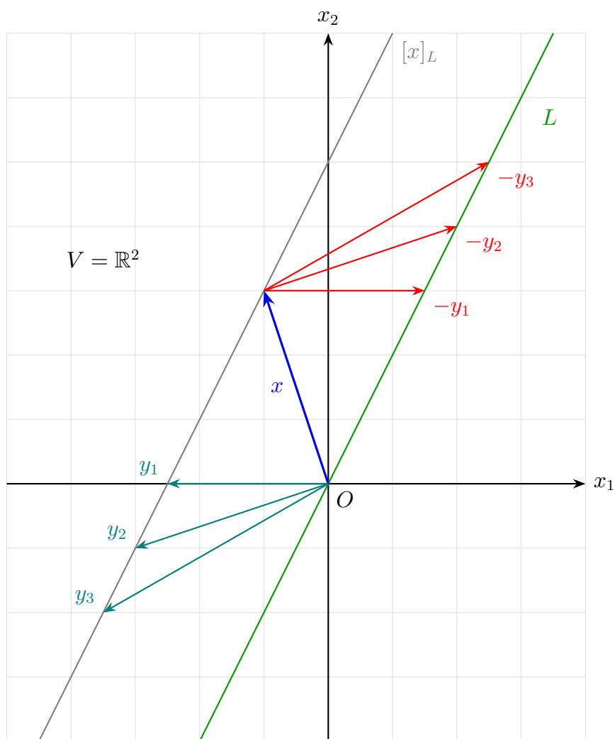
Slika 11.4: x = (-1, 3) , L = \{\alpha(1, 2) \mid \alpha \in \mathbb{R}\} , [x]_L = \{y \in \mathbb{R}^2 \mid x \sim_L y\}
