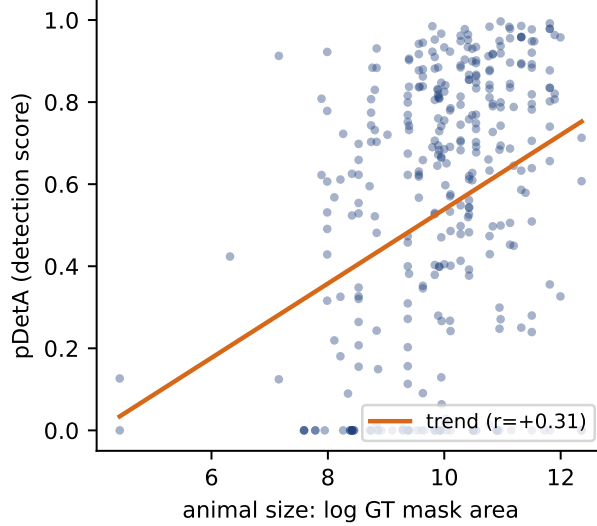
Figure 4.2: The one label-free property that predicts detection: animal size. Per-cell \text{pDetA} rises with the log ground-truth mask area ( r = +0.31 ) — the confound behind the apparent visual-distance effect.
