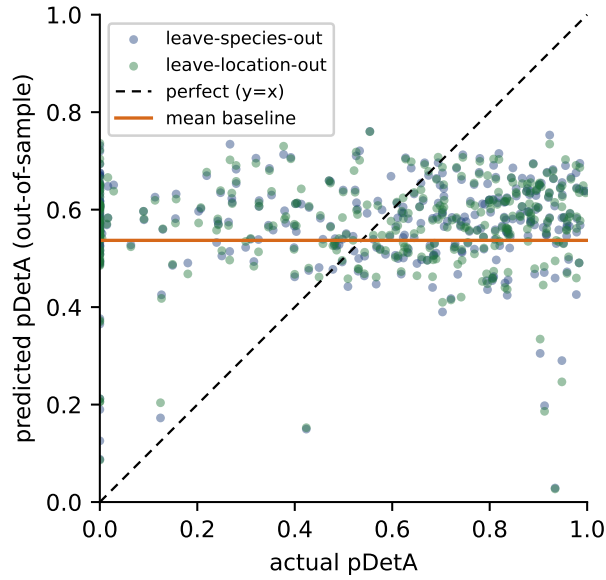
Figure 4.1: Out-of-sample predictions vs the truth for detection (pDetA), on held-out species and locations. The predictions collapse onto the mean baseline (orange) instead of tracking the diagonal (dashed) — the distances carry no out-of-sample predictive power.
