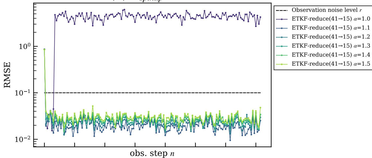
(a) N_{spinup} = 720
