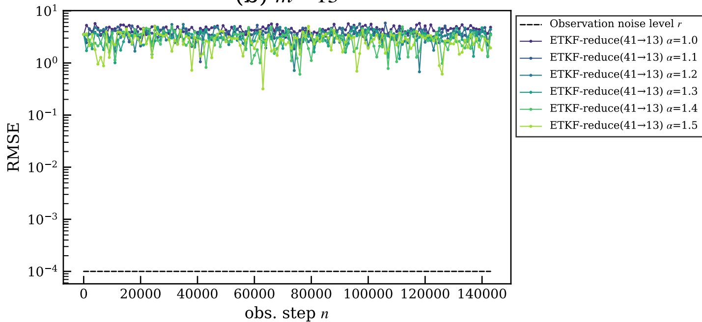
(b) m = 13
