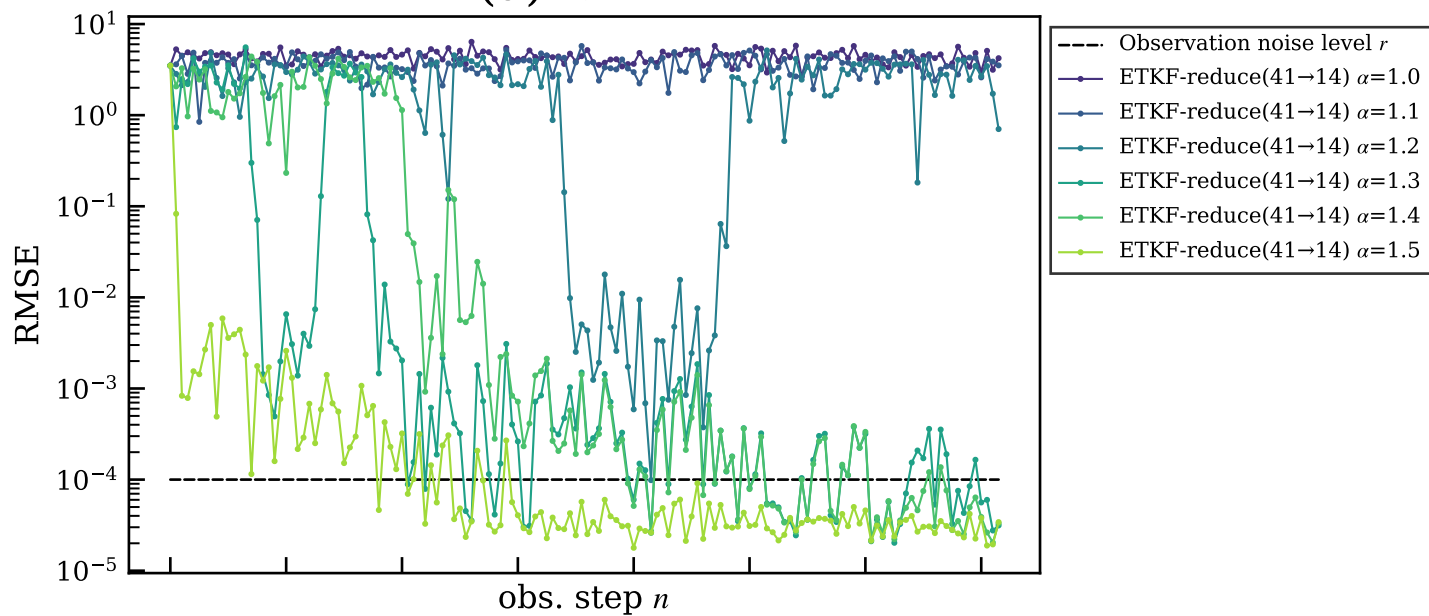
(a) m = 14
