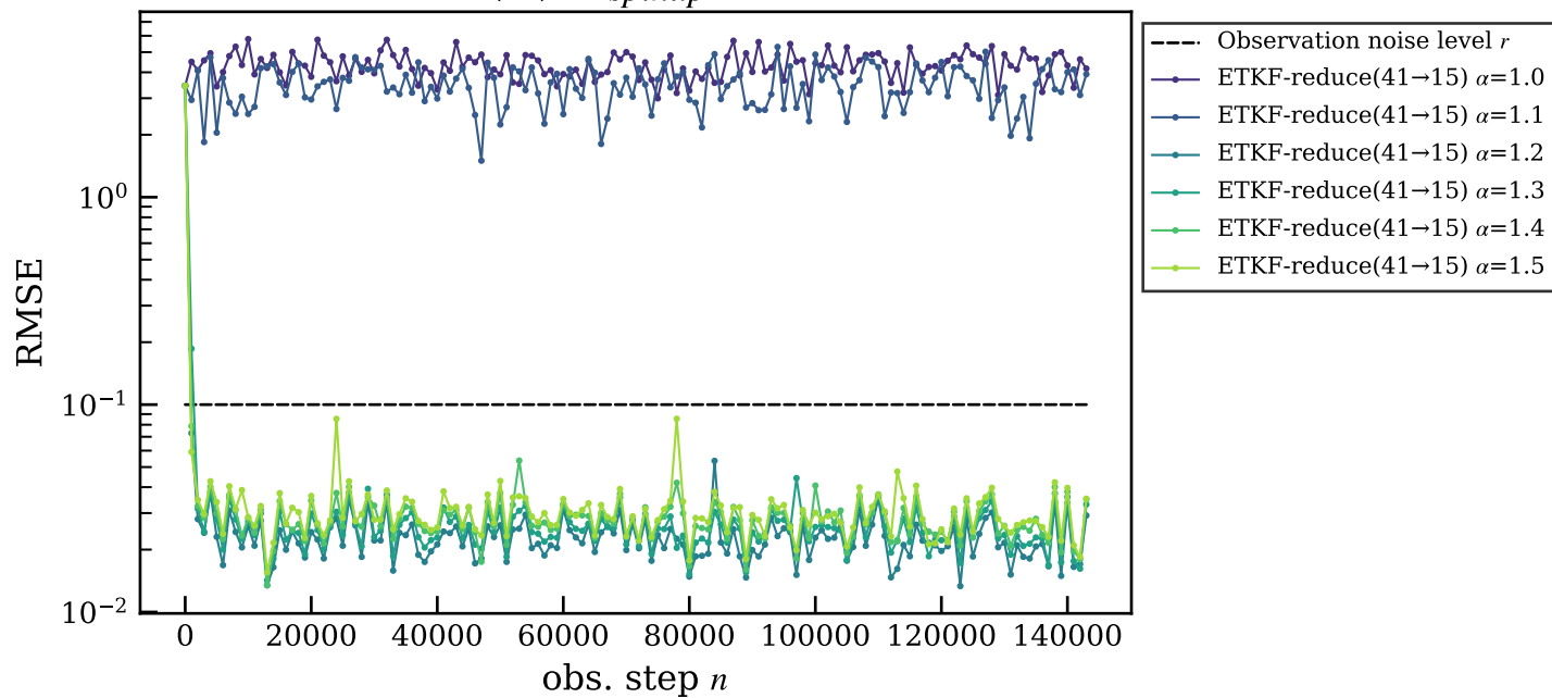
(b) N_{spinup} = 0
