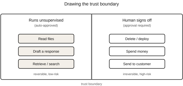
Drawing the trust boundary.
