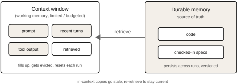
Short-term context and durable memory.
