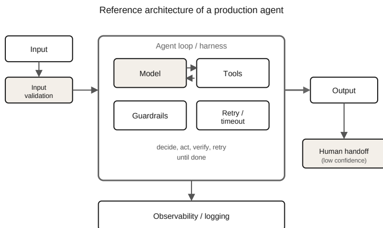
Reference architecture of a production agent.
