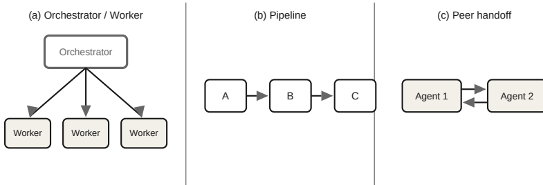
Multi-agent coordination patterns.
