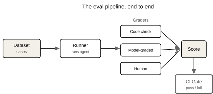
The eval pipeline, end to end.
