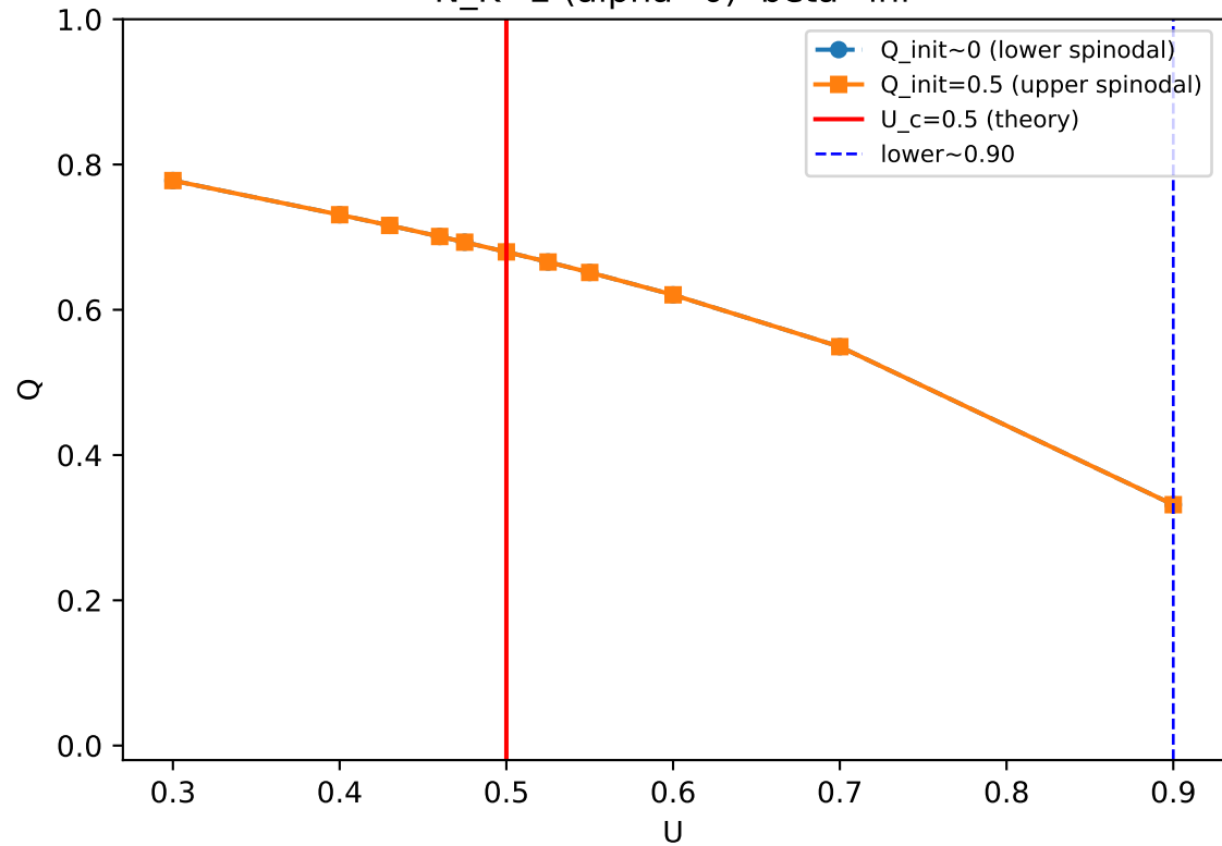
N_K=2 (alpha=0) beta=inf
