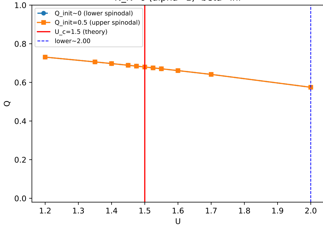
N_K=6 (alpha=1) beta=inf
