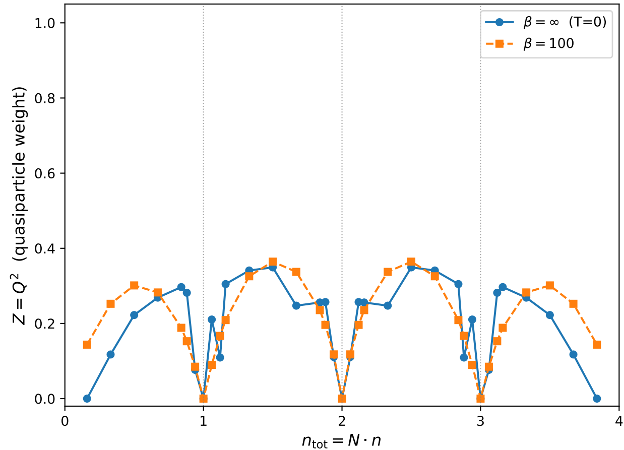
Quasiparticle weight — N=4 , U=4.5
