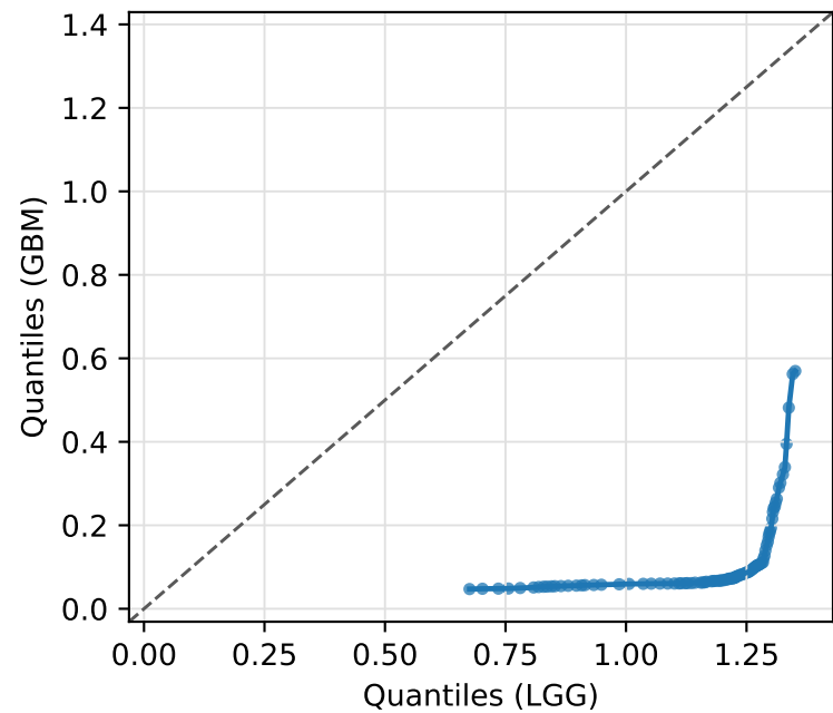
Cell division
