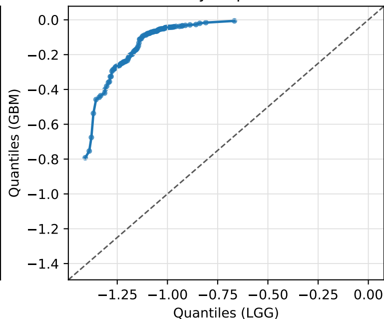
Cell division
