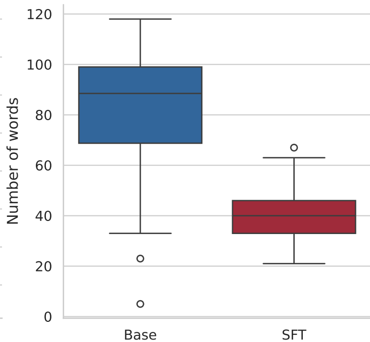
Chain-of-Thought Length
