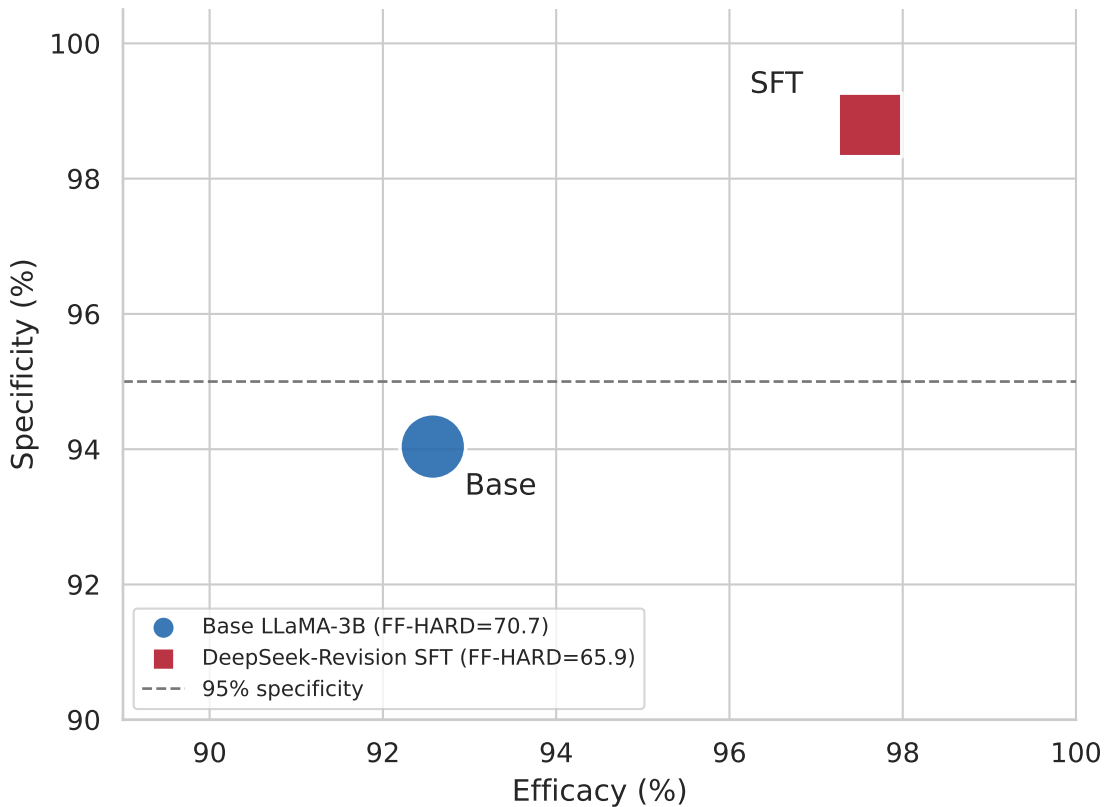
FUR Control Region and Protocol Faithfulness
