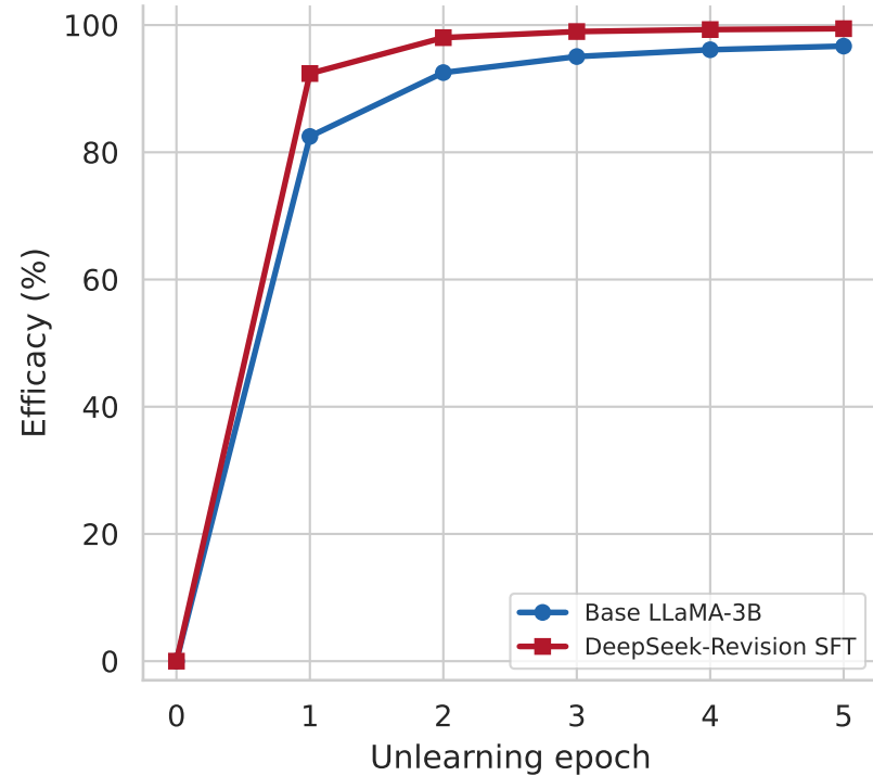
Efficacy Trajectory
