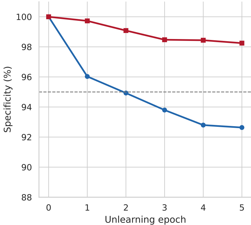
Specificity Trajectory
