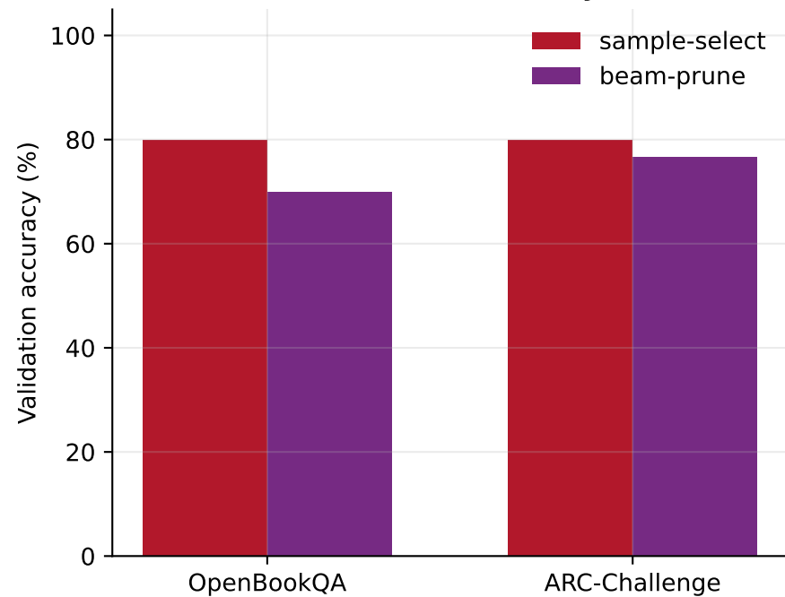
ToT Selector Quality
