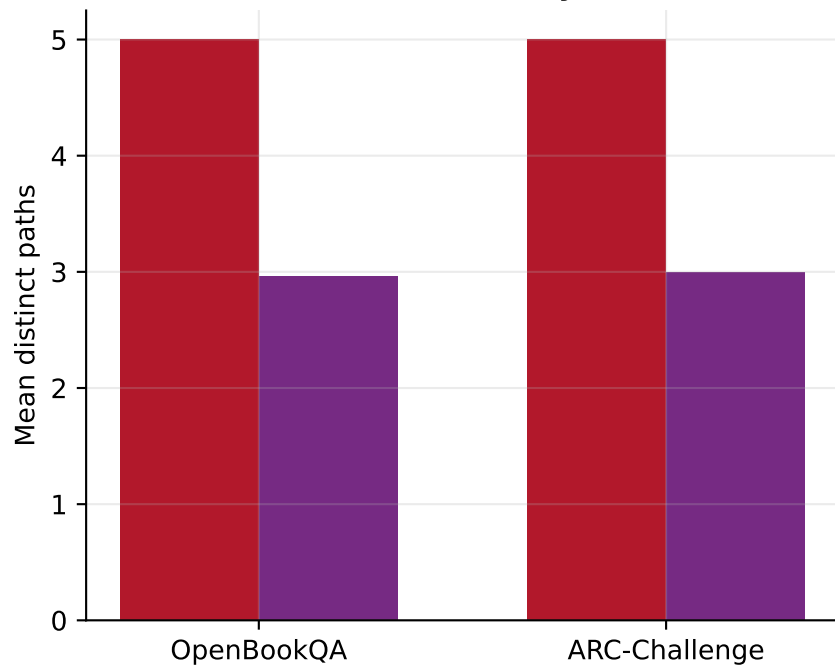
Tree Diversity
