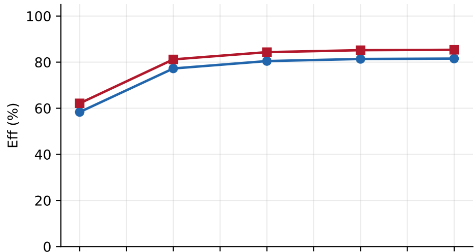
ARC-Challenge
