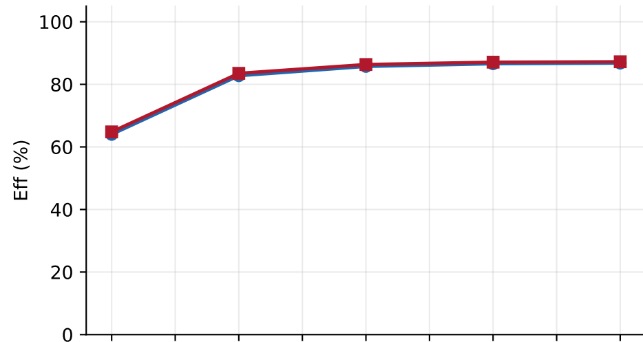
OpenBookQA
