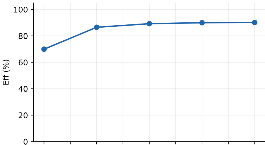
CoT OpenBookQA
