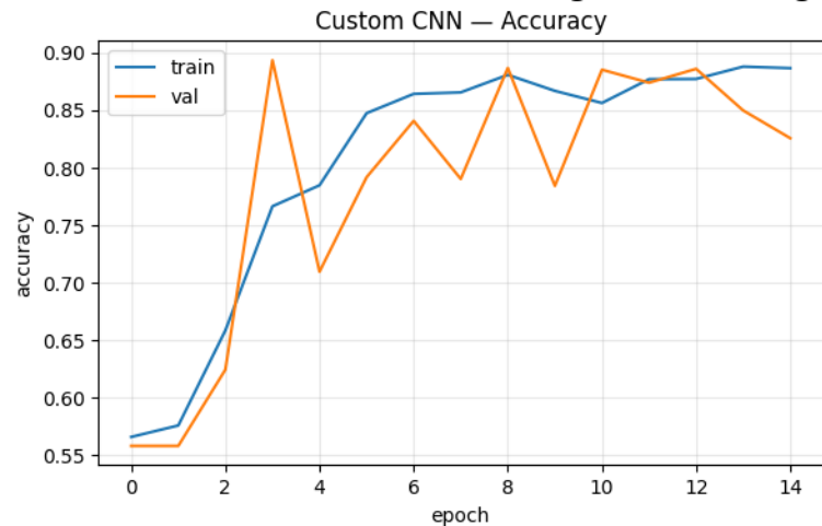
Figure 3: Training & Validation Curves
