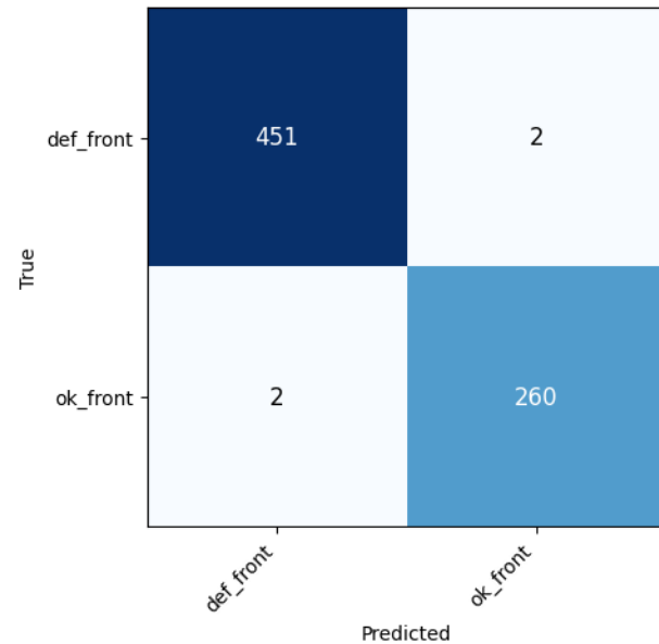
ResNet50
