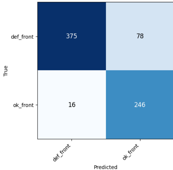
Custom CNN
