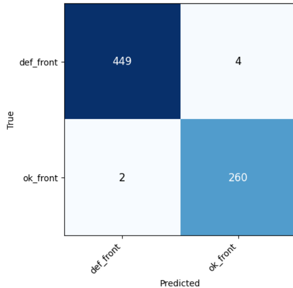
Figure 4: Confusion Matrices MobileNetV2
