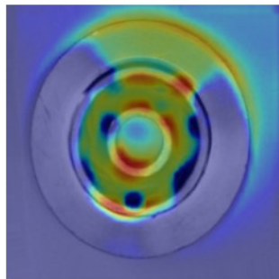
Custom CNN
