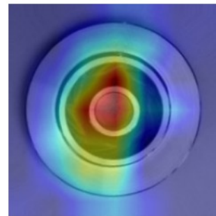
ResNet50
