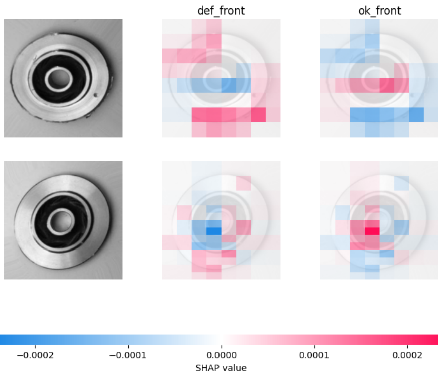
Figure 7: SHAP — ResNet50
